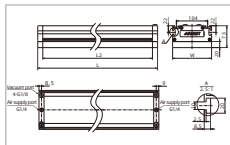
TXC130x1000/1200/1400-A Sponge type
