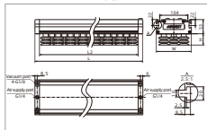
TXC130x1000/1200/1400-B Suction cup type
