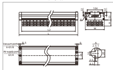
TXC130x400/600/800-B Suction cup type
