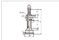
SPJ25-50 Vertical-Pagoda fitting
