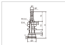
SPJ10-20 Vertical-Pagoda fitting
