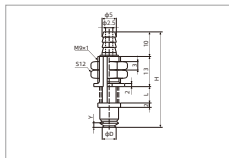
SPJ6-8 Vertical-Pagoda fitting
