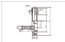
SPF5-8 Lateral-Pagoda fitting
