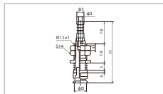
SPF10-20 Vertical-Pagoda fitting
