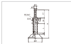
SPF25-50 Vertical-Pagoda fitting
