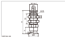
Vertical-One-touch fitting
