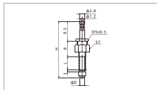
SPF2-3.5 Vertical-Pagoda fitting
