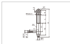
SPF2-3.5 Lateral-Pagoda fitting
