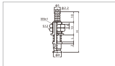
SPF5-8 Vertical-Pagoda fitting
