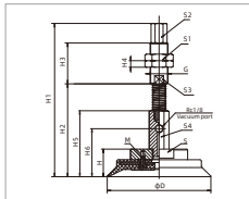
SH40-125 Lateral direction
