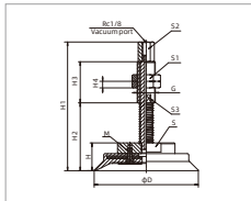
SH40-125 Vertical direction
