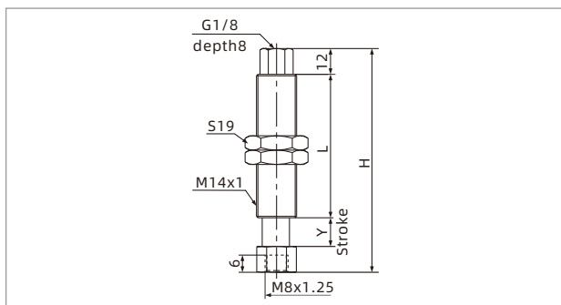
M8F-Vertical female thread connection
