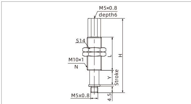
M5M-Vertical male thread connection
