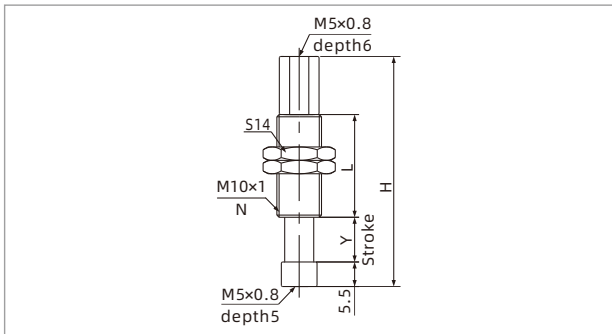
M5F-Vertical female thread connection
