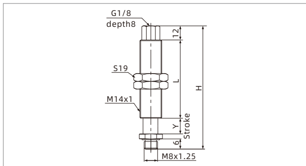
M8M-Vertical male thread connection
