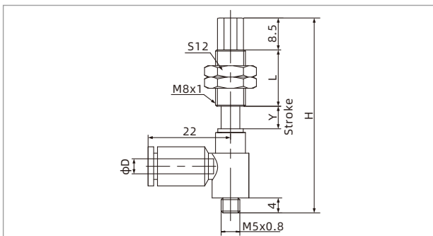
M5M-Lateral male thread connection
