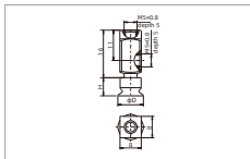
SP3C4-16 Lateral-Female thread connection
