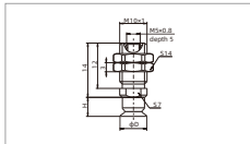
SP3C4-8 Vertical-Male thread connection
