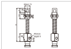
SP3B4-16 Lateral rotating
