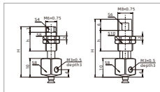
SP3U1.5-3.5 Lateral rotating
