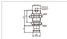
SP3B10□-M5F-M12M
