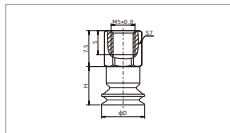
SP3B4-16 F - Female thread connection
