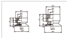
SP3C4-8
