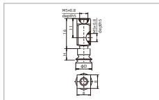
SP3B4□-M5F-M5F
