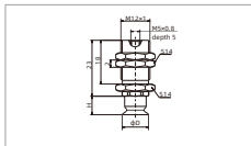
SP3C10-16 Vertical-Male thread connection
