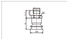
SP3B4-16 M - Male thread connection
