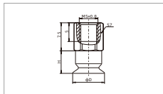
SP3C4-16 F - Female thread connection
