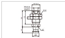
SP3B4□-M5F-M10M
