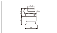
SP3C4-16 M - Male thread connection
