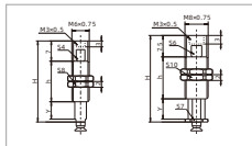
SP3U1.5-3.5 Vertical rotating
