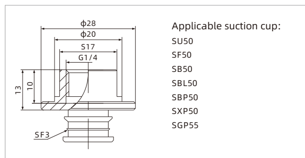
PJS-G2F-SF3
