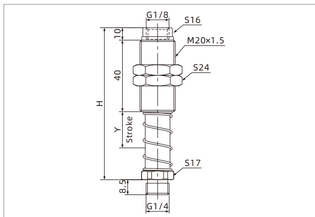
PSPH-E□(R)G2M-M20
