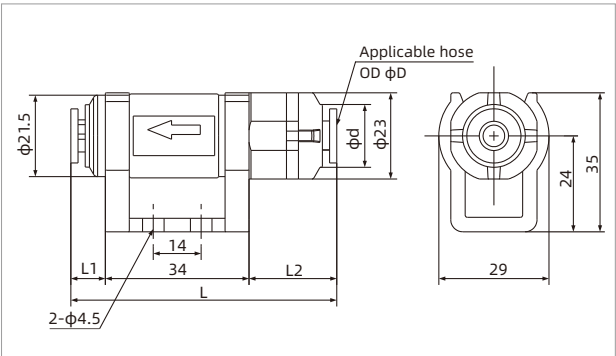
ZFA7□B
