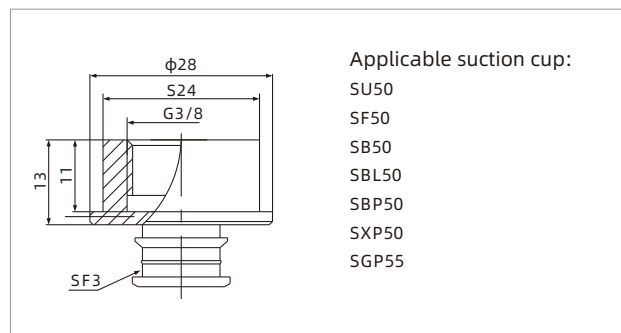
PJS-G3F-SF3
