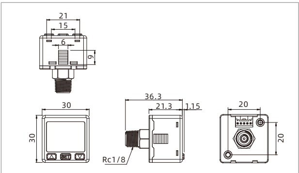
ZPDT-□□-R1M
