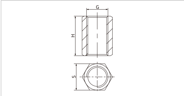
Equal diameter female-female thread
