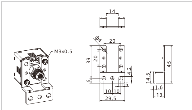
ZPDT-A-MB Mounting bracket A type
