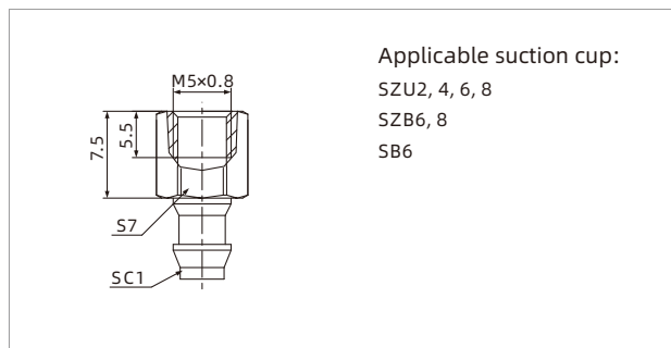
PJS-M5F-SC1
