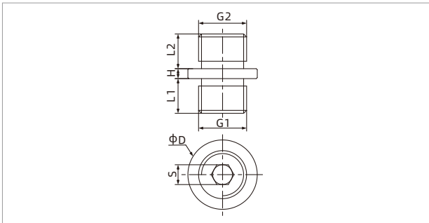
Equal diameter male-male thread
