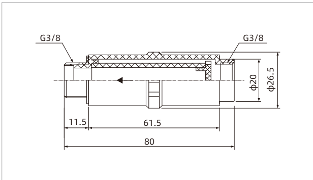
ZFL10
