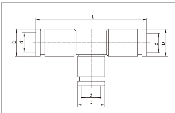
PJP-QT-□
