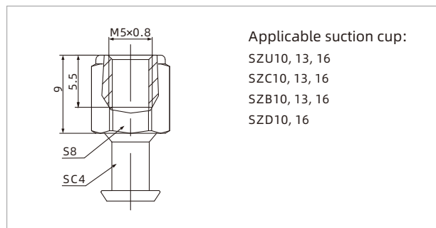
PJS-M5F-SC4
