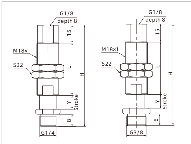
PSPT-I□G2M-M18-H
