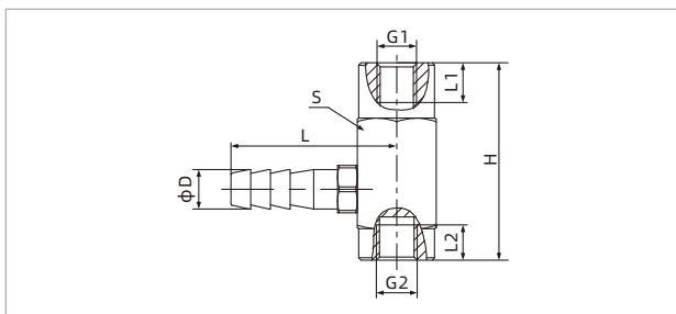
Lateral pagoda fitting
