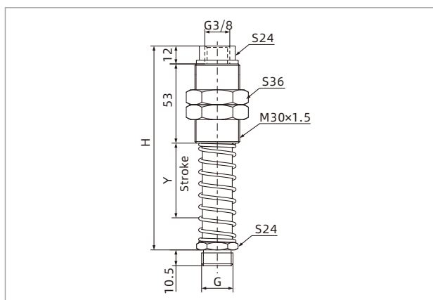
PSPH-E□(R)G3M-M30
