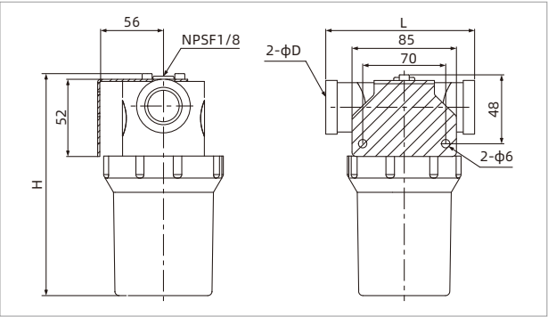
ZFB25B ZFB40B
