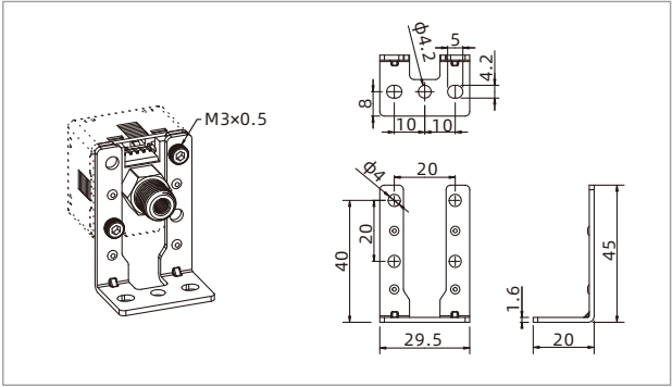
ZPDT-B-MB Mounting bracket B type
