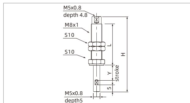
PSPS-I□M5F-M8
