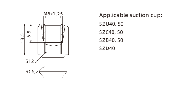
PJS-M8F-SC6
