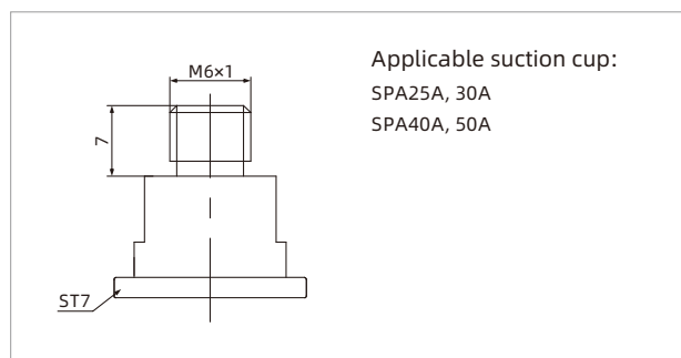
PJS-M6M-ST7
