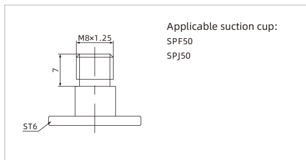
PJS-M8M-ST6
