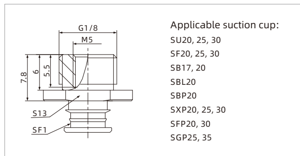
PJS-G1M-SF1
