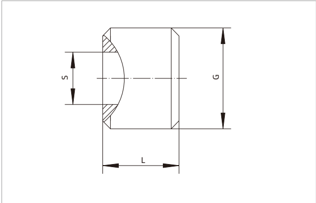
PDA-I-□
