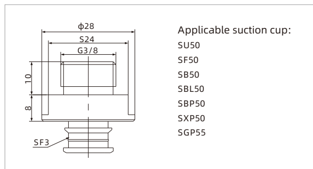
PJS-G3M-SF3
