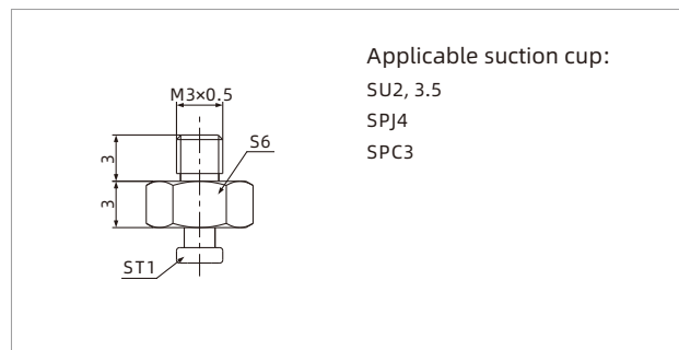
PJS-M3M-ST1
