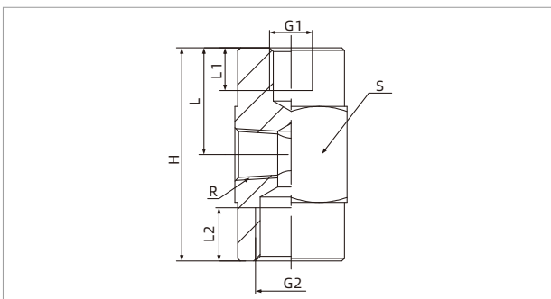
Lateral female thread
