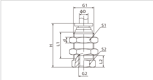
Vertical one-touch fitting
