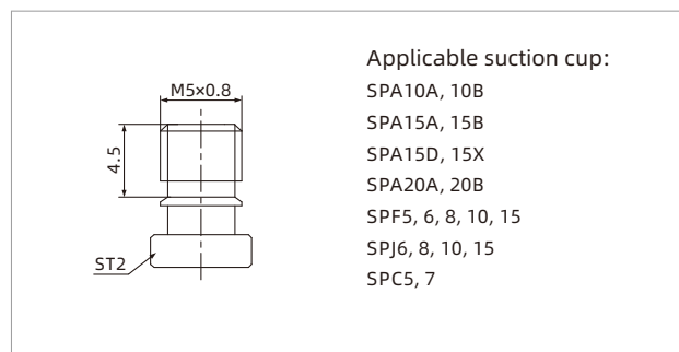
PJS-M5M-ST2
