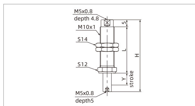
PSPS-I□M5F-M10
