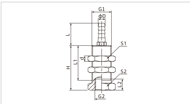
Vertical pagoda fitting
