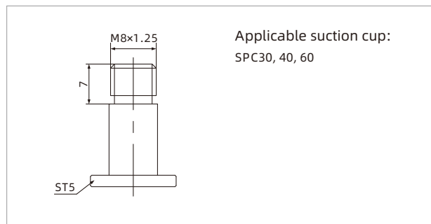
PJS-M8M-ST5
