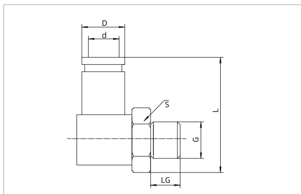
PJP-L-A8-□
