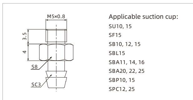
PJS-M5M-SC3
