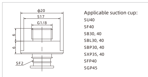
PJS-G1M-SF2
