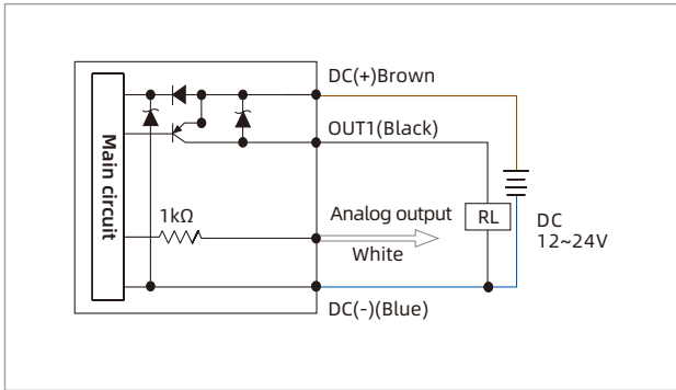
ZPDT-□PV-R1M 1PNP+Analog voltage output (1-5V)
