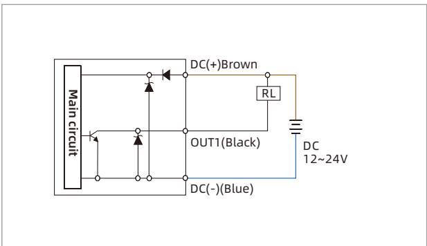
ZPDE-□N-R1M 1NPN output
