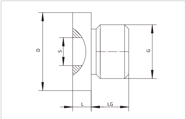
PDA-L-□
