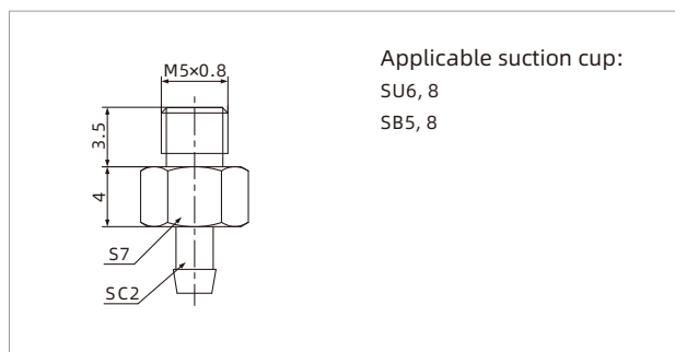
PJS-M5M-SC2
