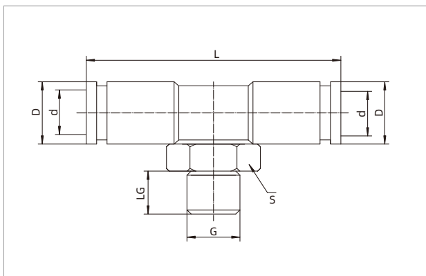
PJP-T-A8-□
