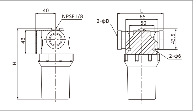
ZFB10(15-20)B
