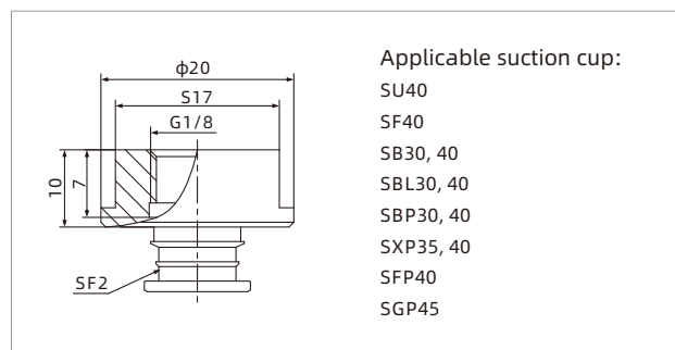
PJS-G1F-SF2
