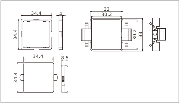
ZPDT-PC Front protective lid + panel adapter
