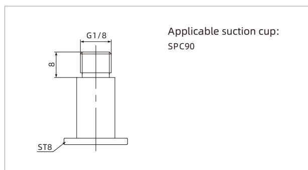
PJS-G1M-ST8
