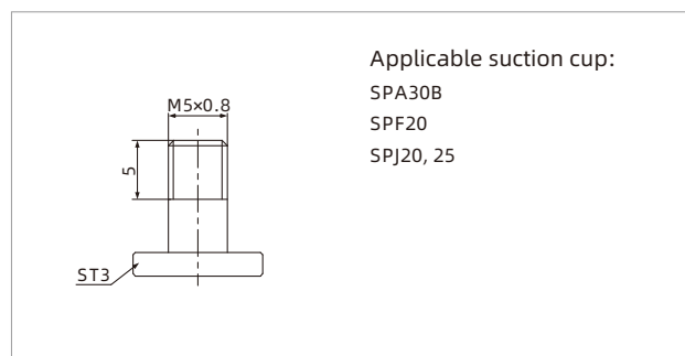
PJS-M5M-ST3
