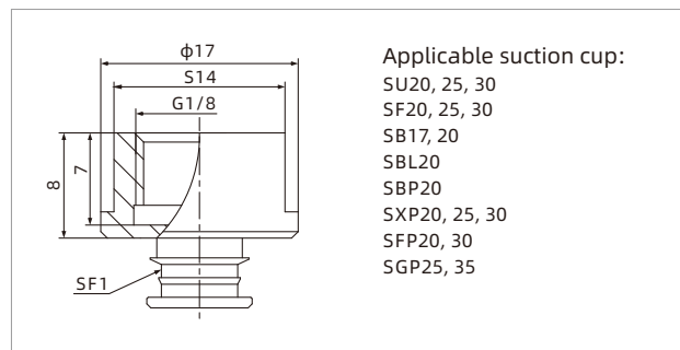
PJS-G1F-SF1
