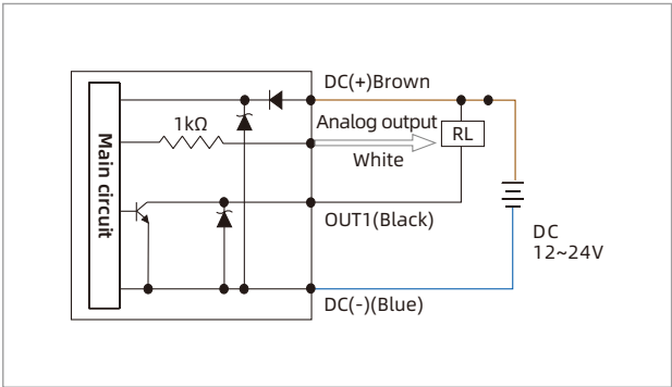
ZPDT-□NV-R1M 1NPN+Analog voltage output (1-5V)
