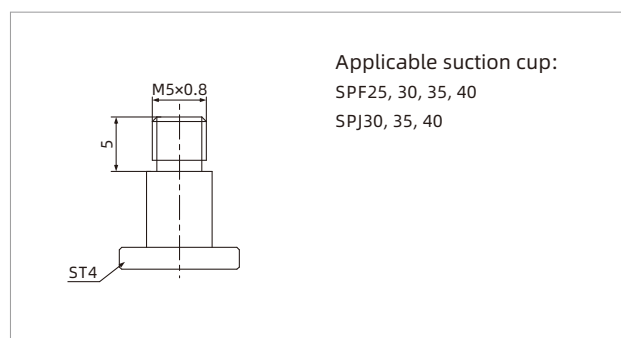
PJS-M5M-ST4
