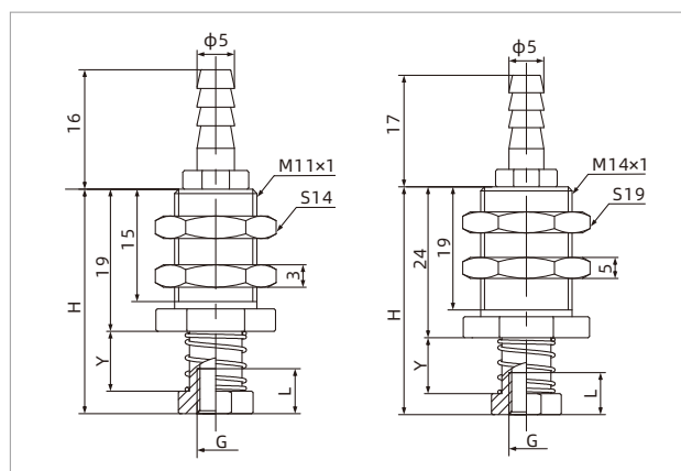
PSPF-E□B6M5F-M11
