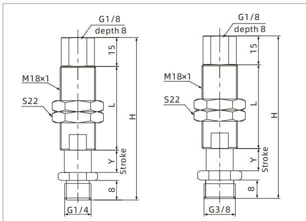
PSPT-I□G2M-M18
