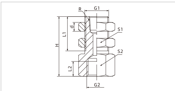
Vertical female thread
