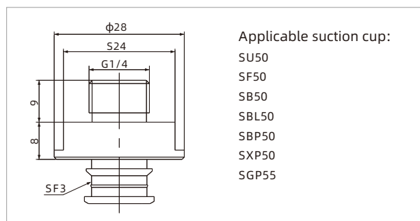
PJS-G2M-SF3
