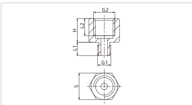
Different diameter female-male thread
