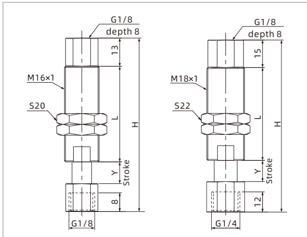
PSPT-I□G1F-M16
