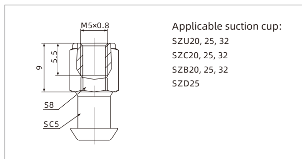
PJS-M5F-SC5
