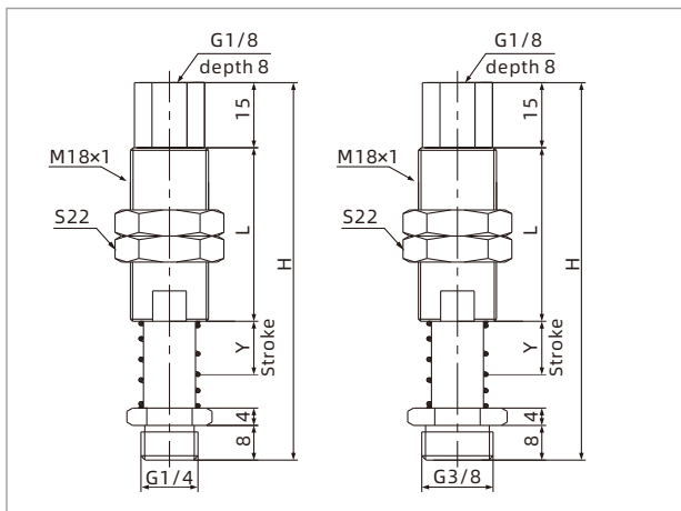
PSPT-E□G2M-M18
