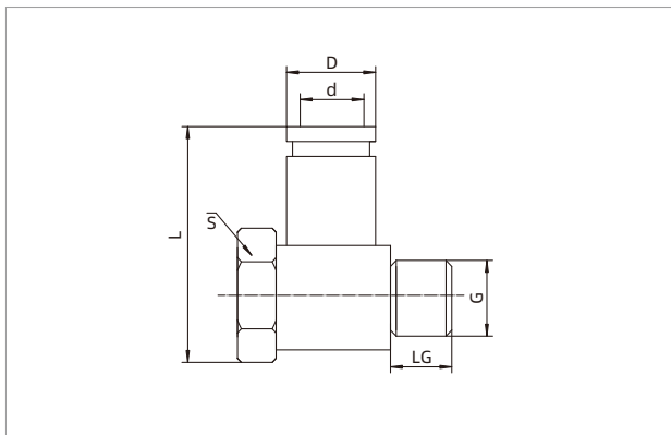
PJP-LT-A8-□
