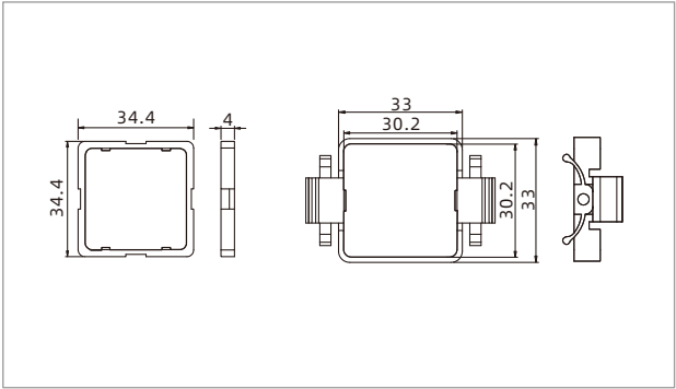
ZPDT-PS Panel adapter
