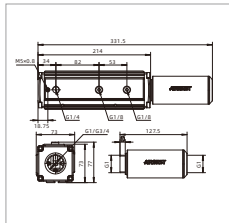
AMD-□-LG8-□ type (Straight exhaust)
