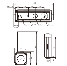
AMD-□-LG6-□ type (Side exhaust)
